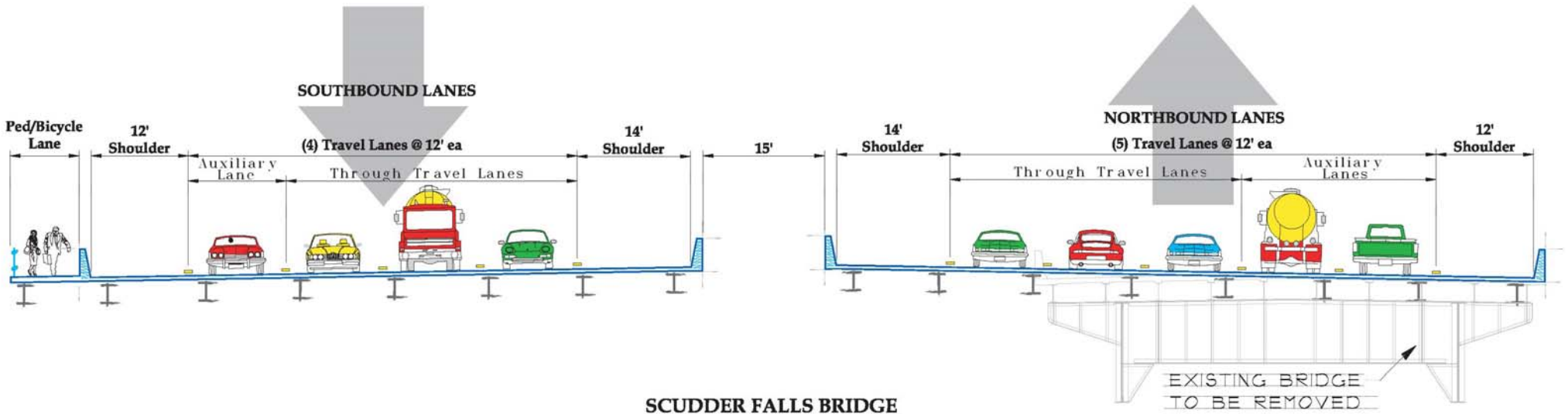
SCUDDER FALLS BRIDGE UPSTREAM ALTERNATIVE
