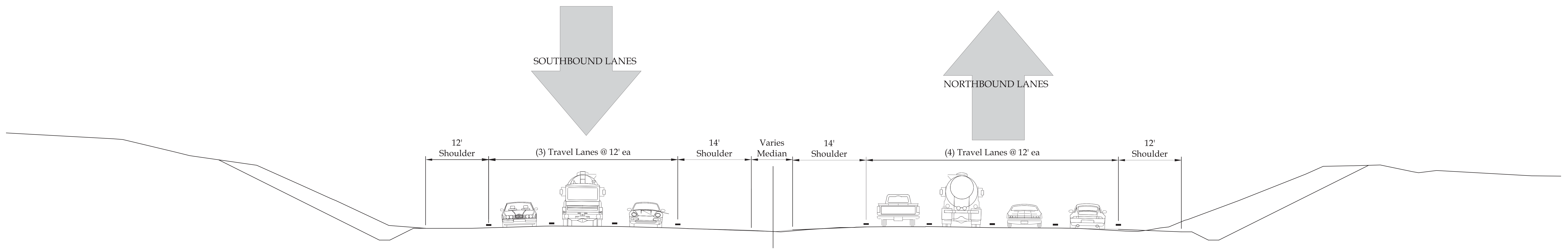
I-95 NEW JERSEY PROPOSED ROADWAY SECTION TYPICAL SECTION WIDENING NORTHBOUND
